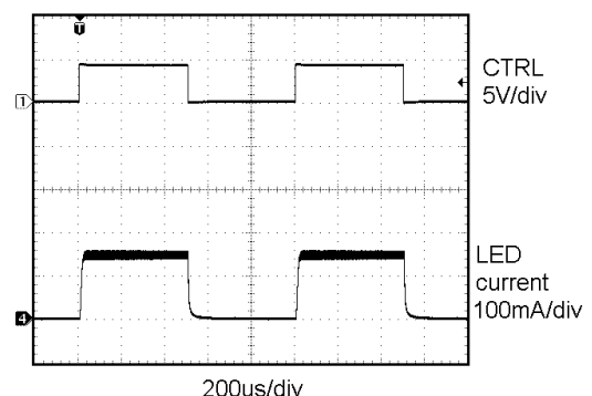
Figure 24. PWM at 1 kHz on CTRL Pin
