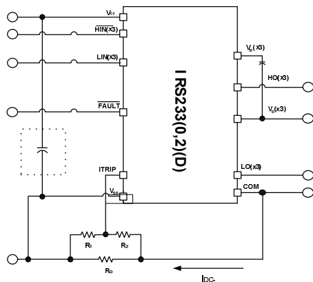
Figure 35: Supply capacitor
