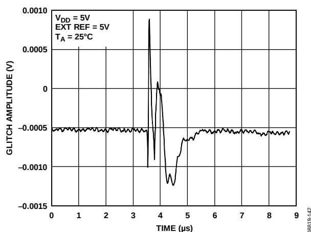
Figure 36. Analog Crosstalk
