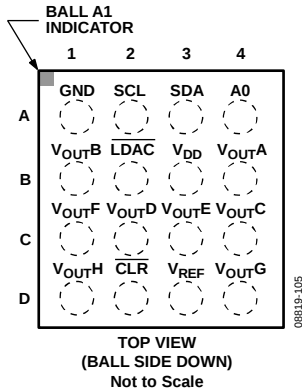
Figure 5. 16-Ball WLCSP
