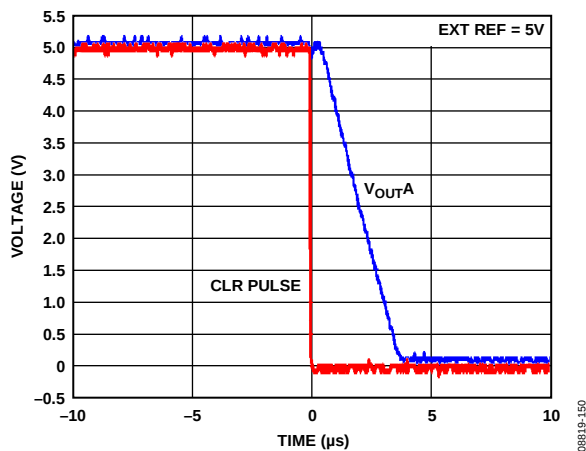
Figure 44. Hardware \overline{CLR}
