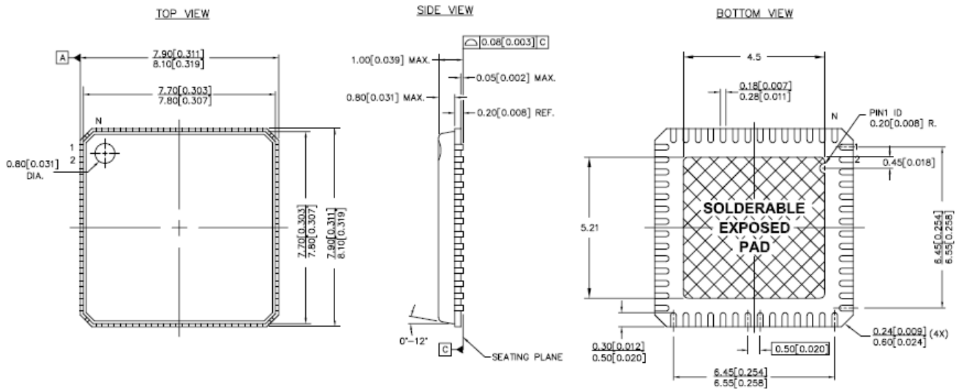
Figure 9. 56-Pin (8x8 mm) QFN-MLF (PUNCH)
