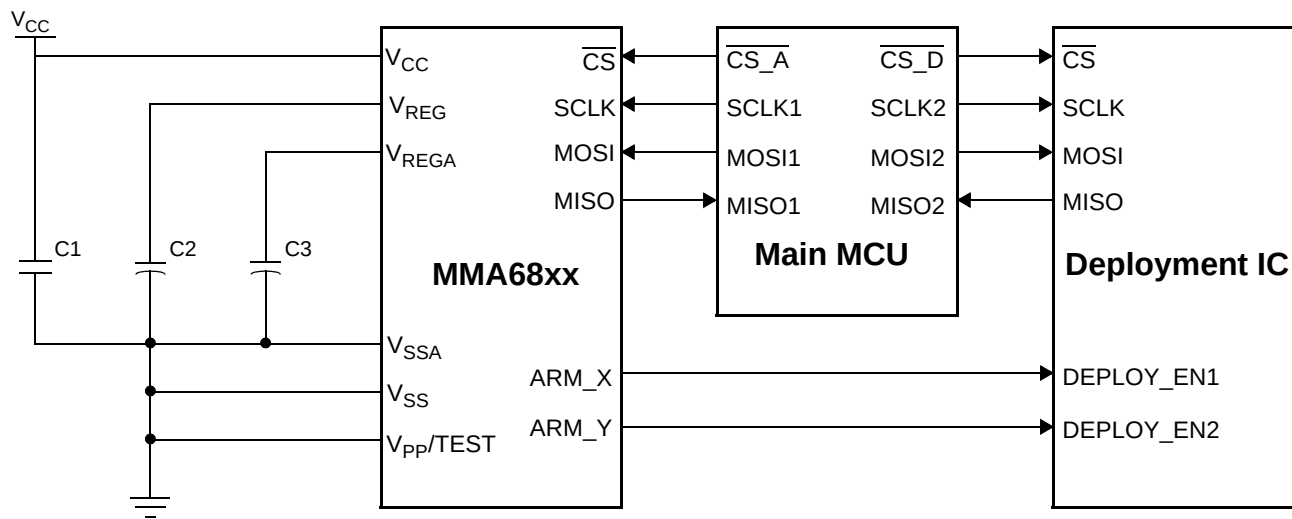
Figure 1. Application Diagram
