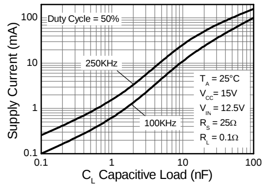
Supply Current
