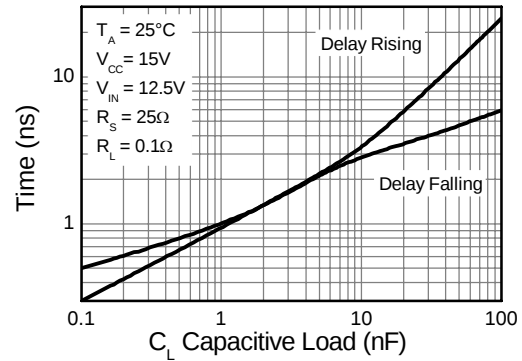
Propagation Delay
