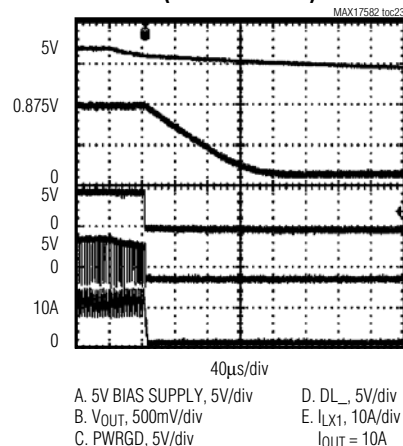
BIAS SUPPLY REMOVAL (UVLO RESPONSE)
