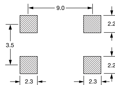
Figure 3) Land Pattern
