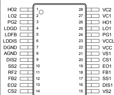
PW PACKAGE (Top View)
