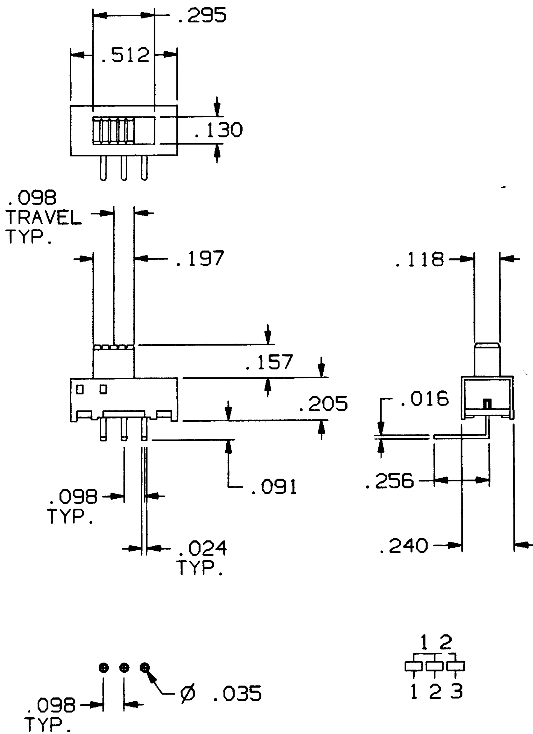
STS121RA PC LAYOUT TOLERANCE: \pm .002
