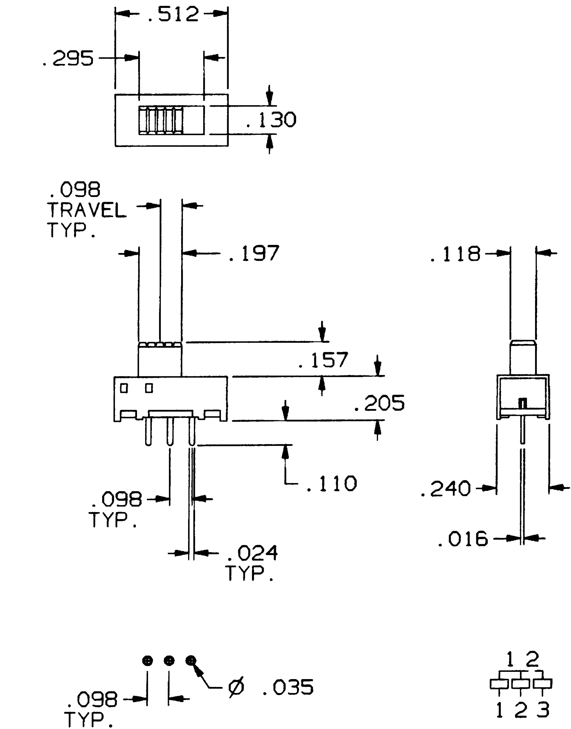
STS121PC PC LAYOUT TOLERANCE: \pm .002
