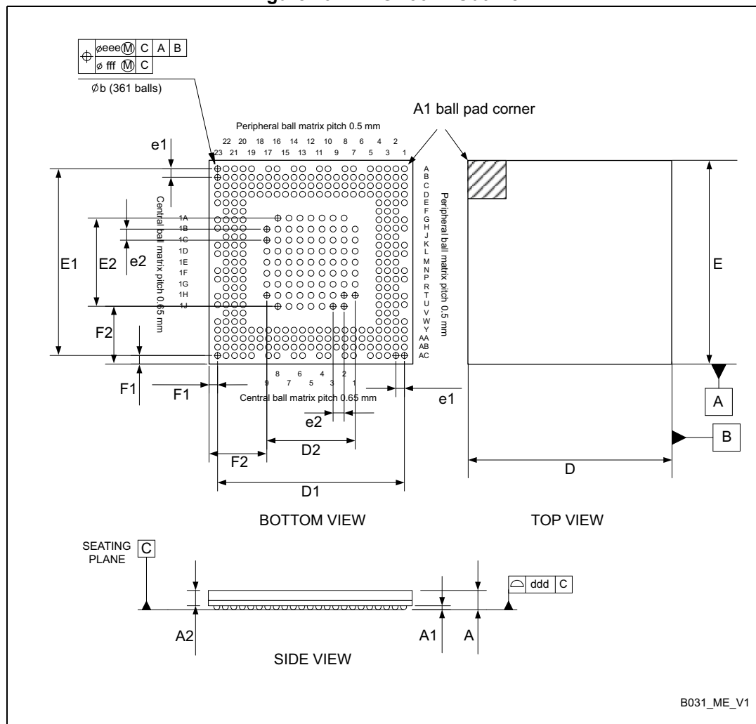
Figure 70. TFBGA361 - Outline
