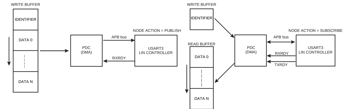
Figure 32-53. Master Node with PDC (PDCM = 0)
