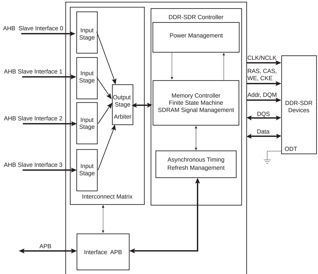
Figure 21-1. DDRSDRC Module Diagram
