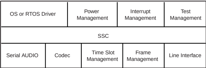
Figure 33-3. Application Block Diagram
