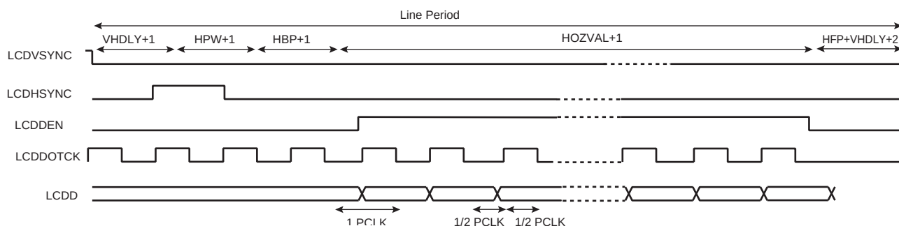
Figure 47-7. TFT Panel Timing (Line Expanded View), CLKMOD = 1
