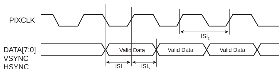
Figure 48-21. ISI Timing Diagram
