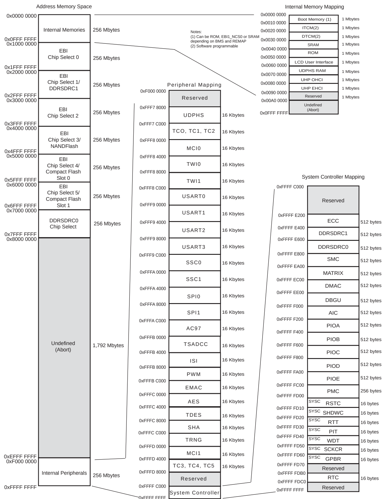
Figure 5-1. SAM9G46 Memory Mapping
