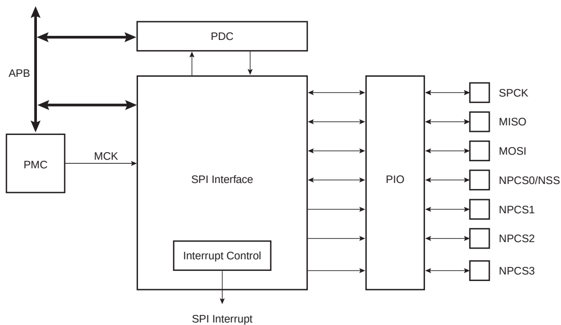
Figure 28-1. Block Diagram
