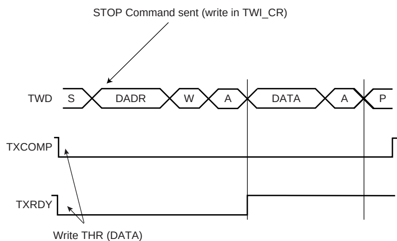
Figure 30-7. Master Write with Multiple Data Bytes
