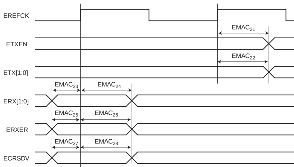
Figure 48-24. EMAC RMII Timings
