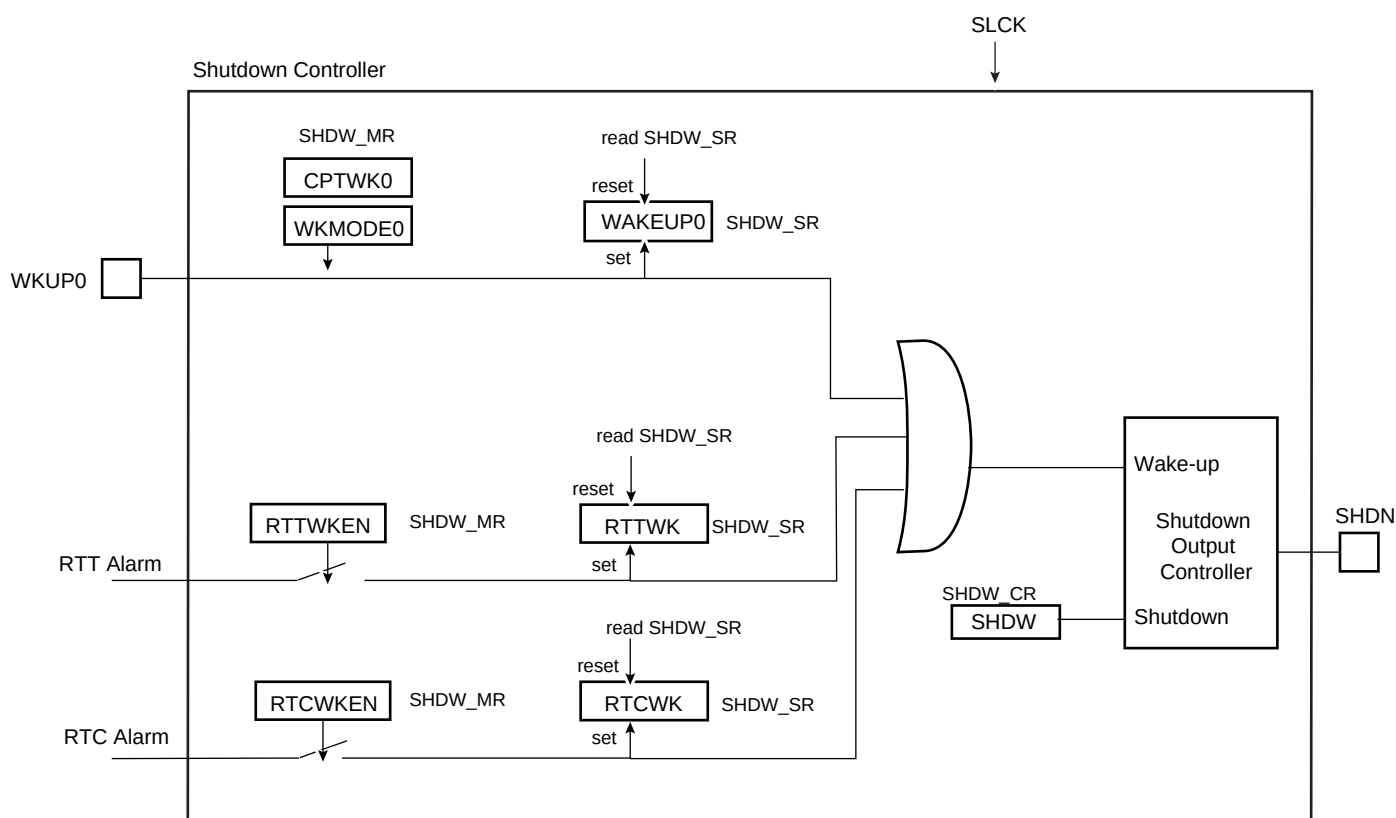
Figure 16-1. Shutdown Controller Block Diagram
