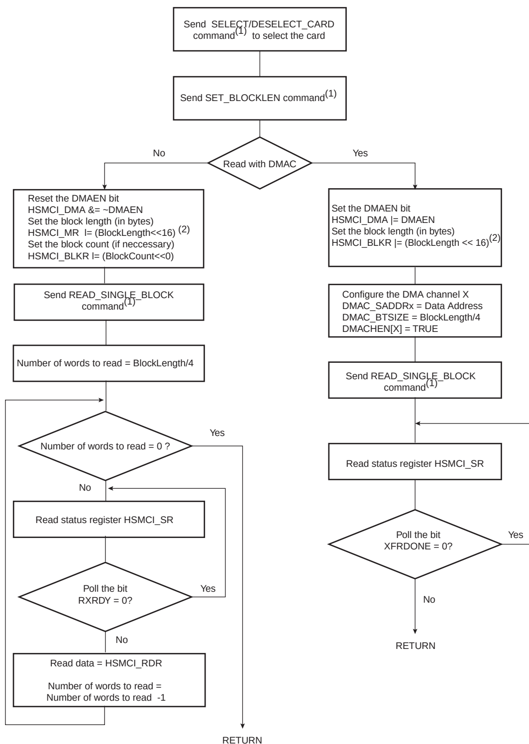
Figure 35-8. Read Functional Flow Diagram
