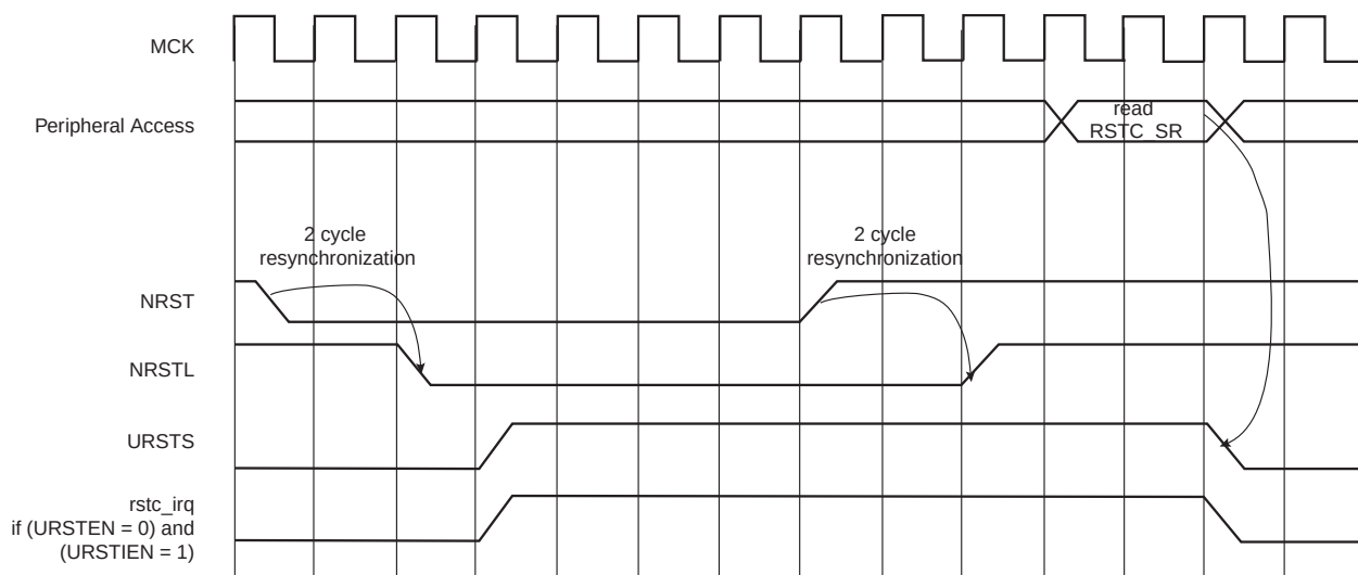
Figure 11-9. Reset Controller Status and Interrupt
