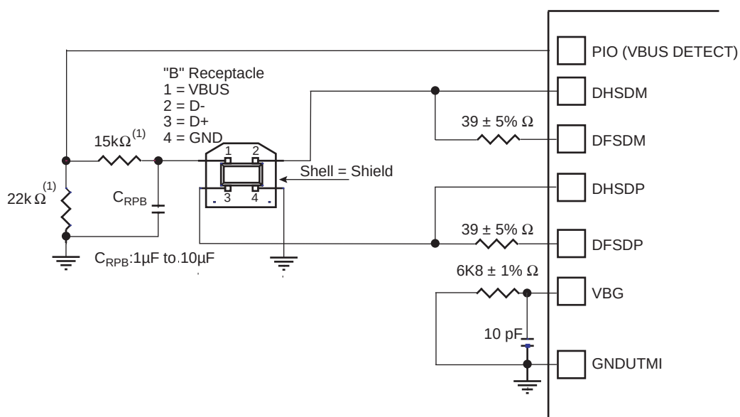
Figure 37-3. Board Schematic
