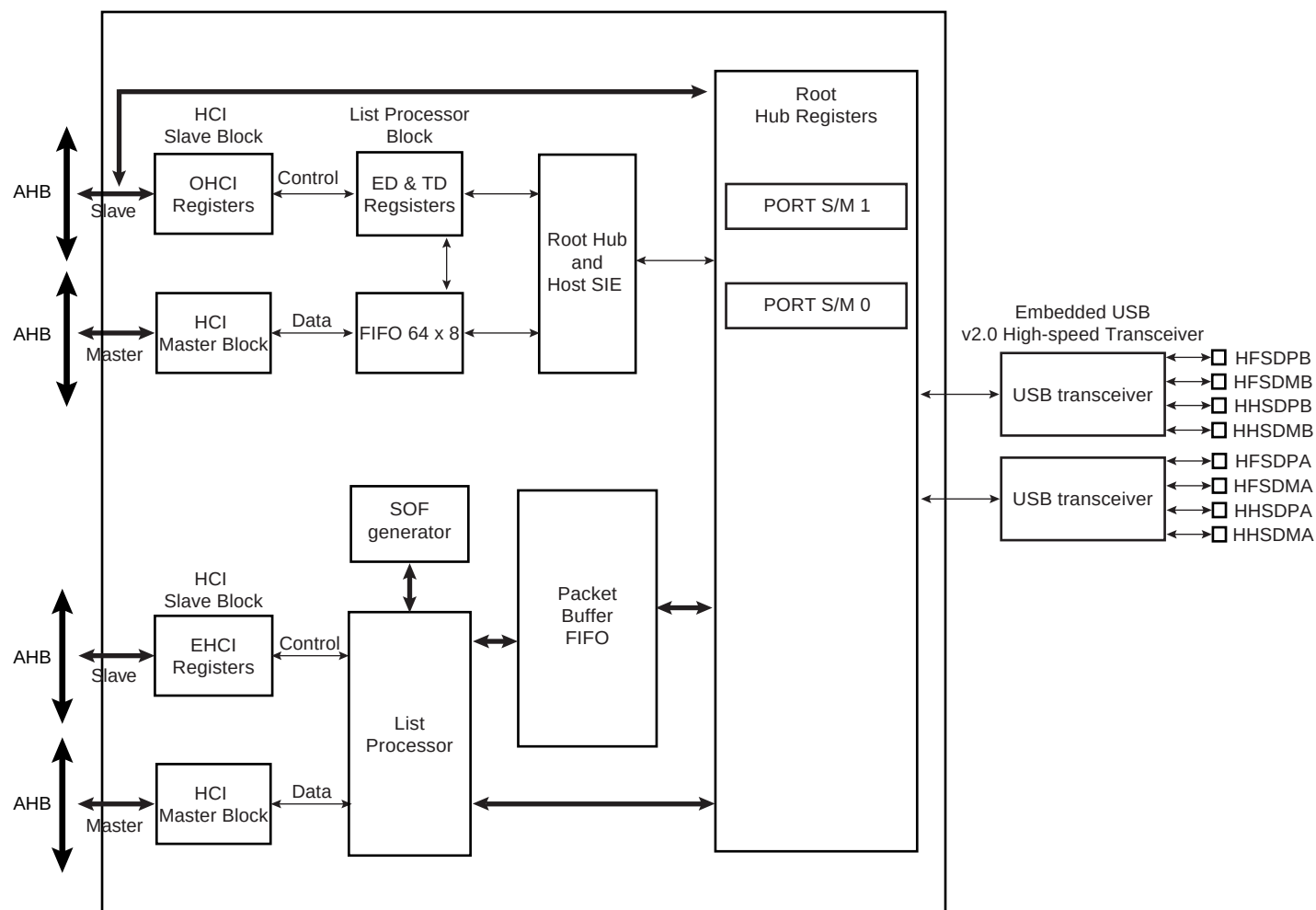
Figure 36-2. Block Diagram
