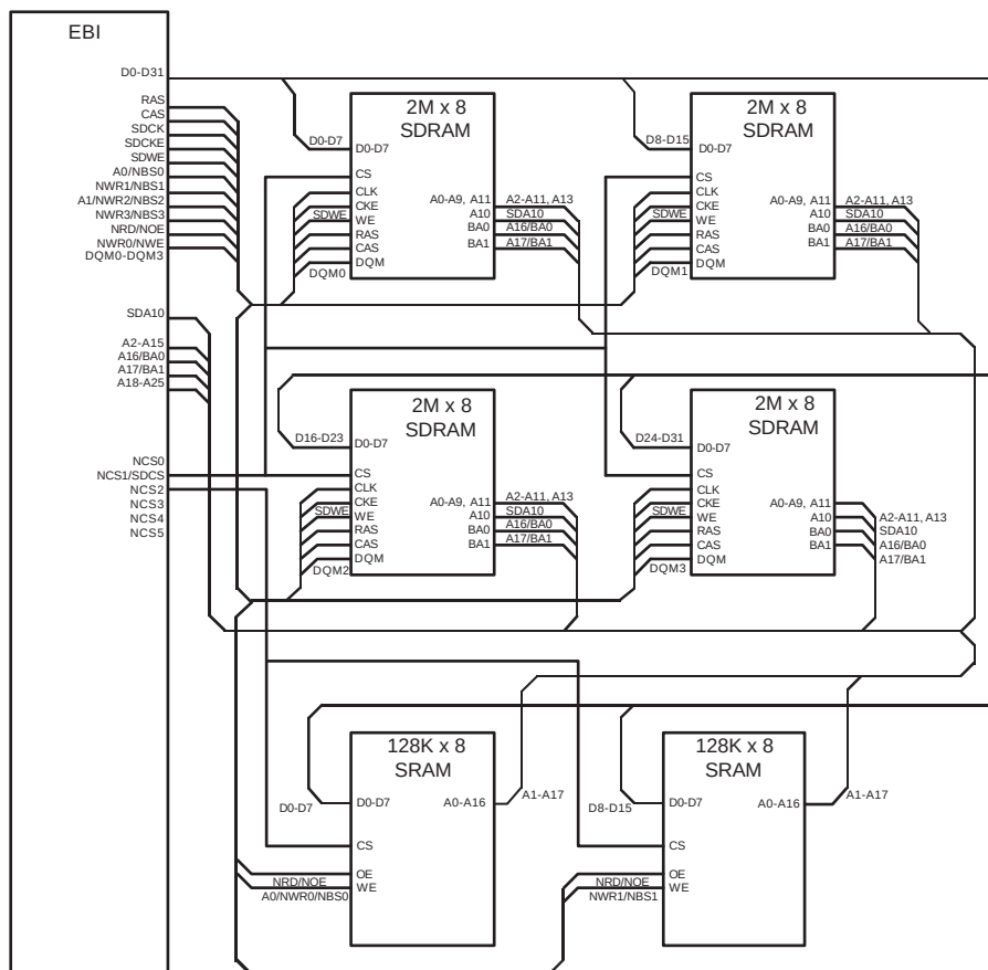
Figure 19-5. EBI Connections to Memory Devices
