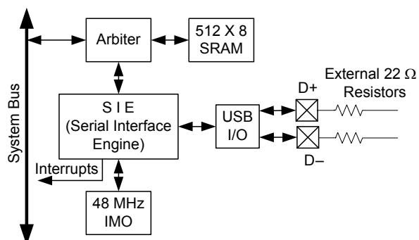
Figure 7-20. USB
