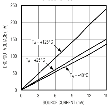
MAX6126_50 DROPOUT VOLTAGE vs. SOURCE CURRENT
