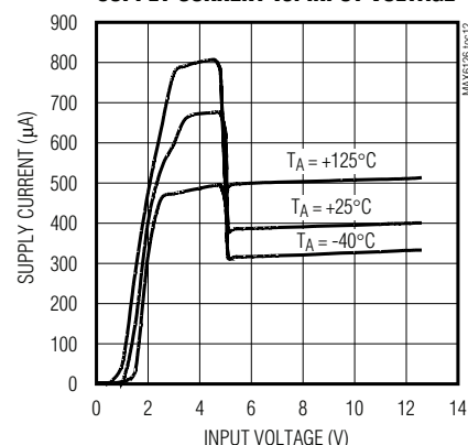
MAX6126_50 SUPPLY CURRENT vs. INPUT VOLTAGE
