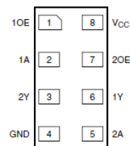
X2-DFN1210-8
