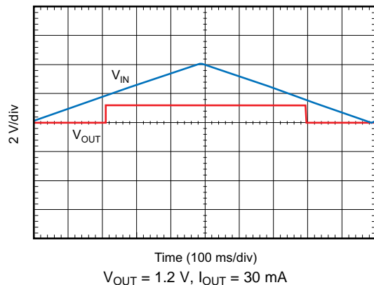
Figure 41. V_{IN} Ramp Up, Ramp Down Response
