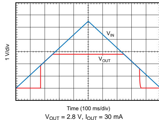
Figure 42. V_{IN} Ramp Up, Ramp Down Response
