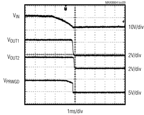
POWER-DOWN WAVEFORMS
