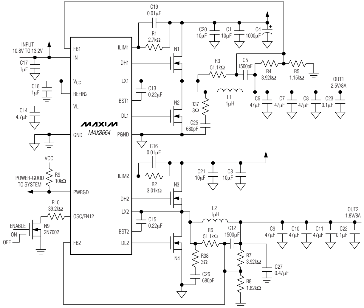
Figure 2. Low-Cost, 600kHz Typical Application Circuit
