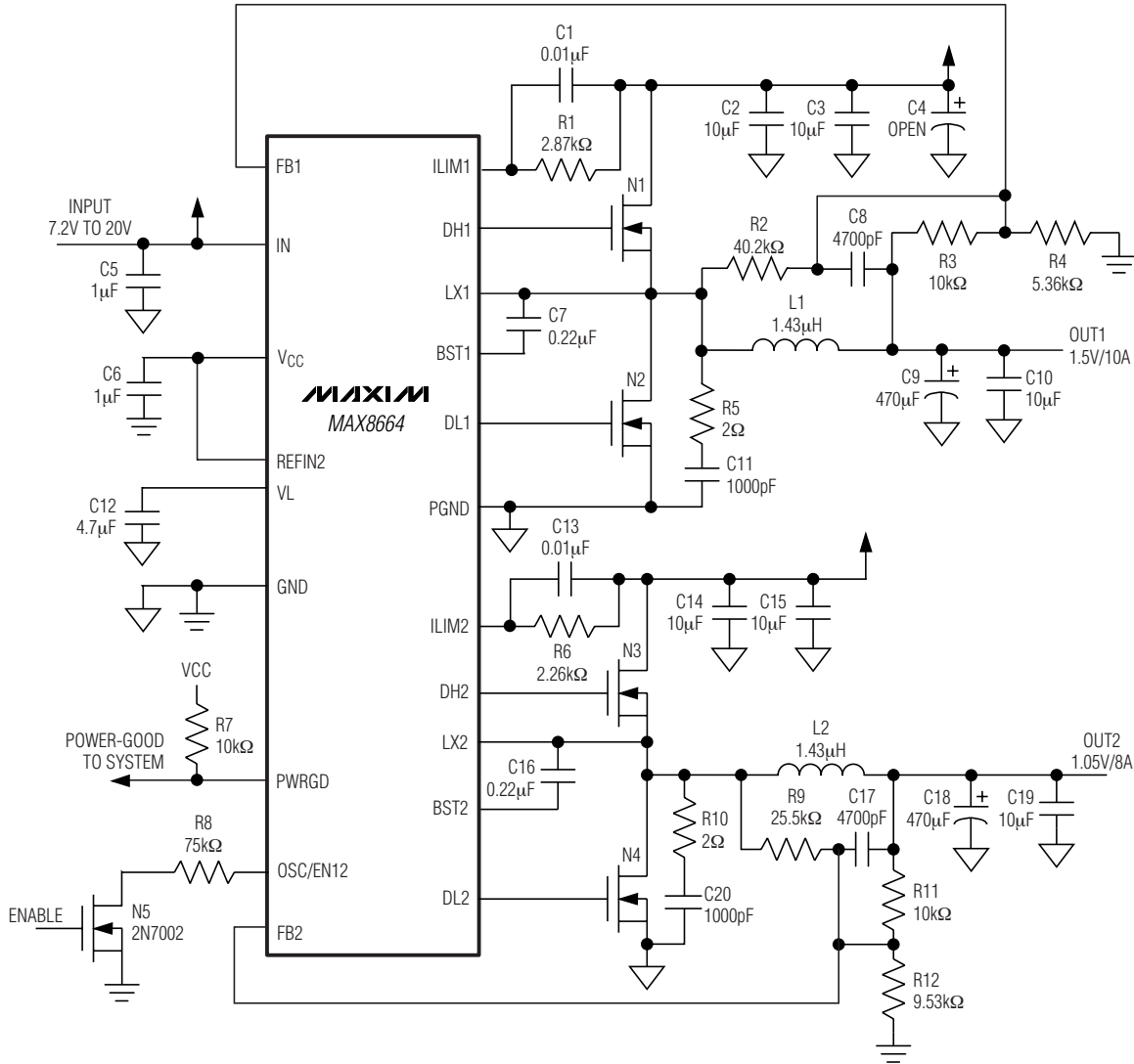
Figure 5. 300kHz Circuit with 7.2V to 20V Input
