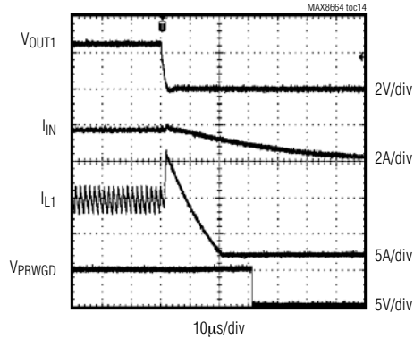
SHORT-CIRCUIT WAVEFORMS
