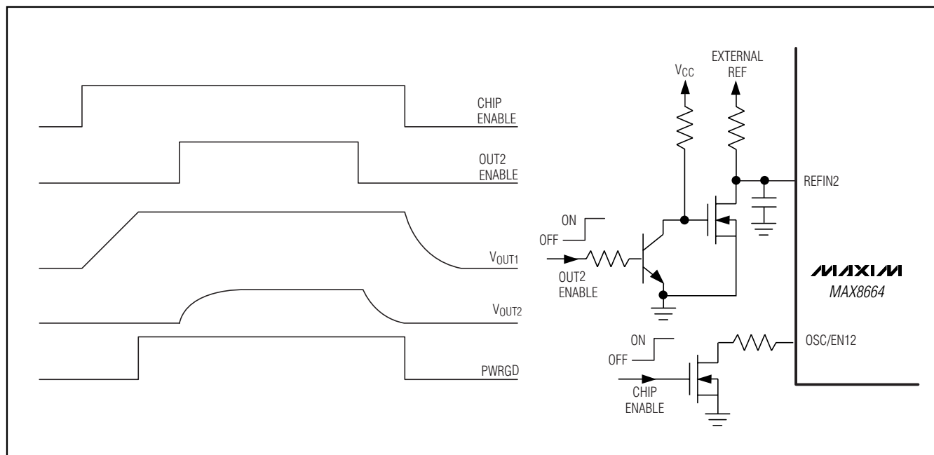
Figure 6d. Sequencing Startup and Shutdown Waveforms with System Enable 2 Signal
