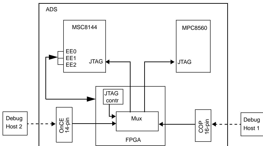
Figure 5-12. JTAG Multiplexing
