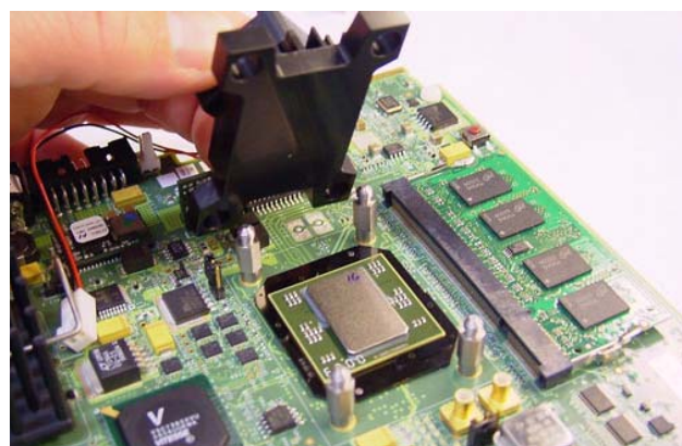
Figure 7-4. Remove Heat Sink
