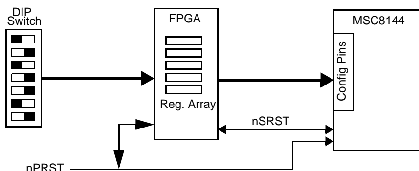
Figure 5-9. Configuration Scheme
