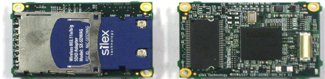
Figure 1 SX-560-1701 top and bottom view
