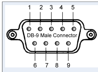
Figure 7 Serial Port DB-9 Connector
