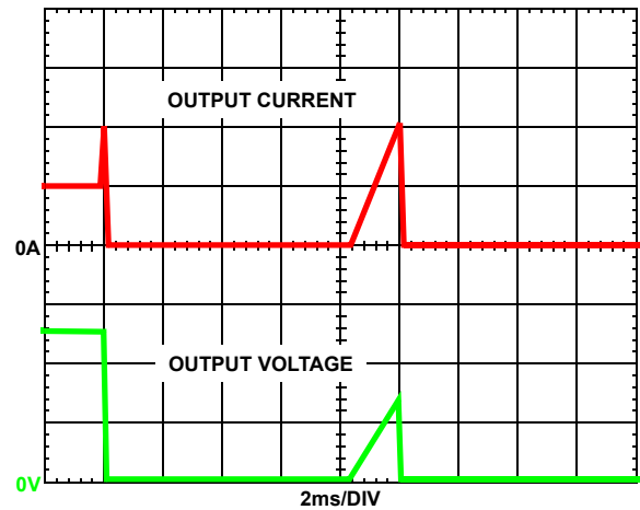
FIGURE 14. OVERCURRENT BEHAVIOR IN HICCUP MODE f_{sw} = 500kHz
