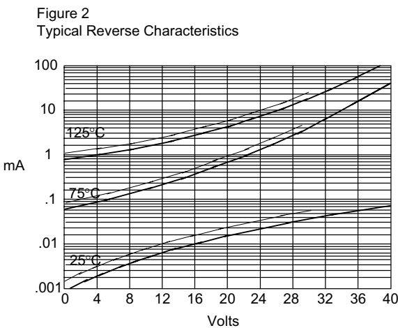
Typical Reverse Current - mA versus Reverse Voltage - Volts
