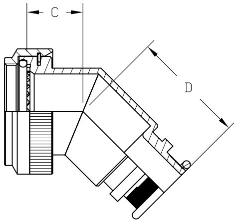
45° ADAPTER-TYPE I
