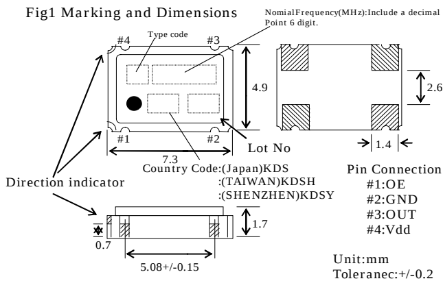
Fig1 Marking and Dimensions
