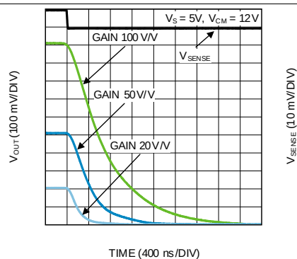
Figure 15. Large Step Response
