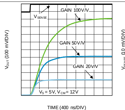
Figure 16. Small Step Response
