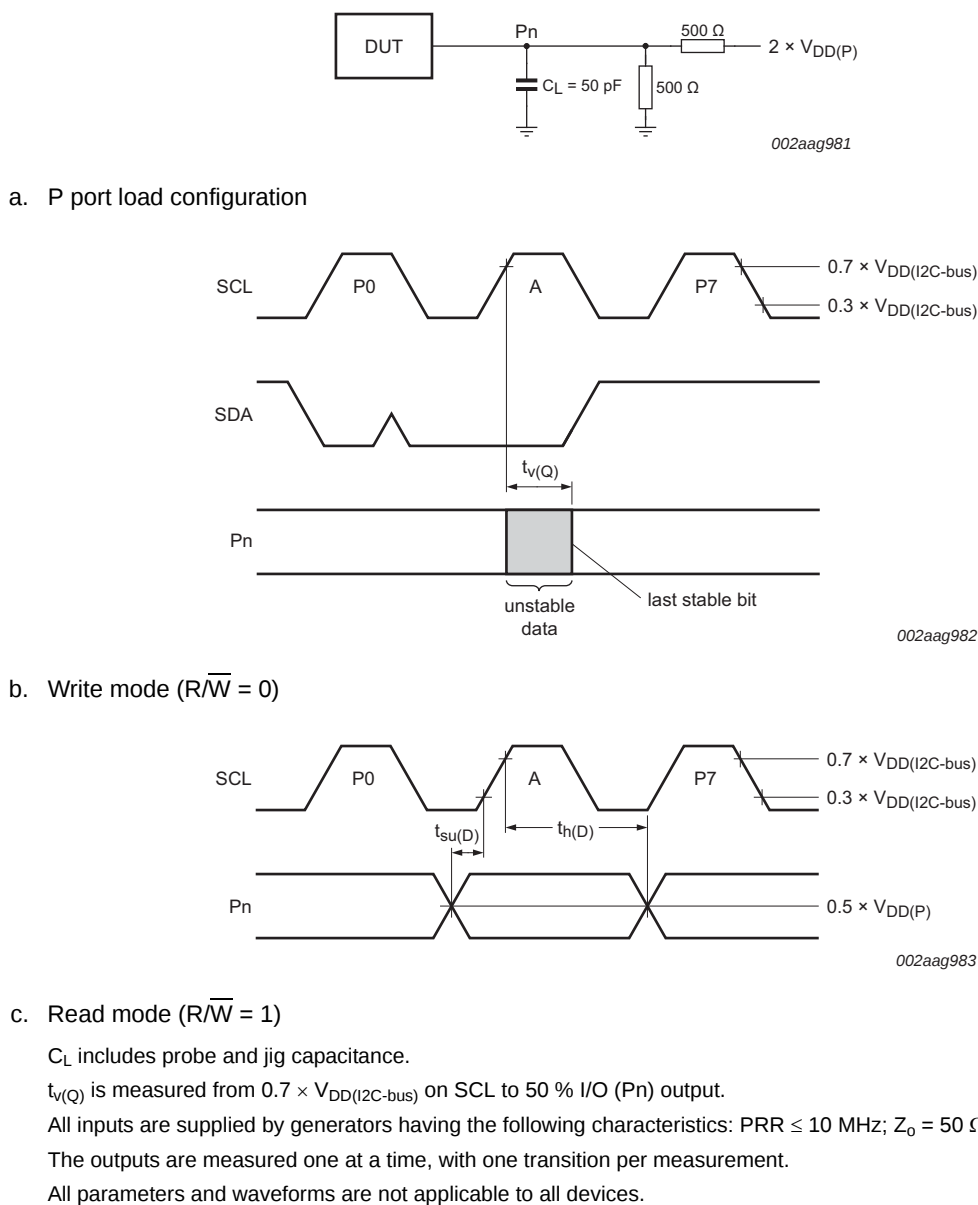
Fig 38. P port load circuit and voltage waveforms
