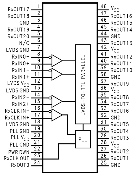
Figure 3. DS90CR218
