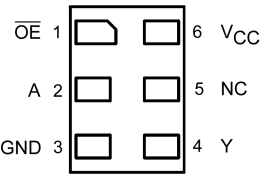
Pad Assignments for MicroPak
