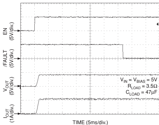
Current-Limit Response
