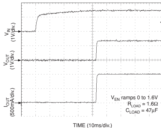
UVLO Response
