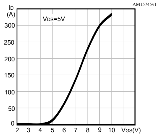
Figure 8. Transfer characteristics
