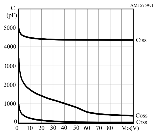
Figure 12. Capacitance variations
