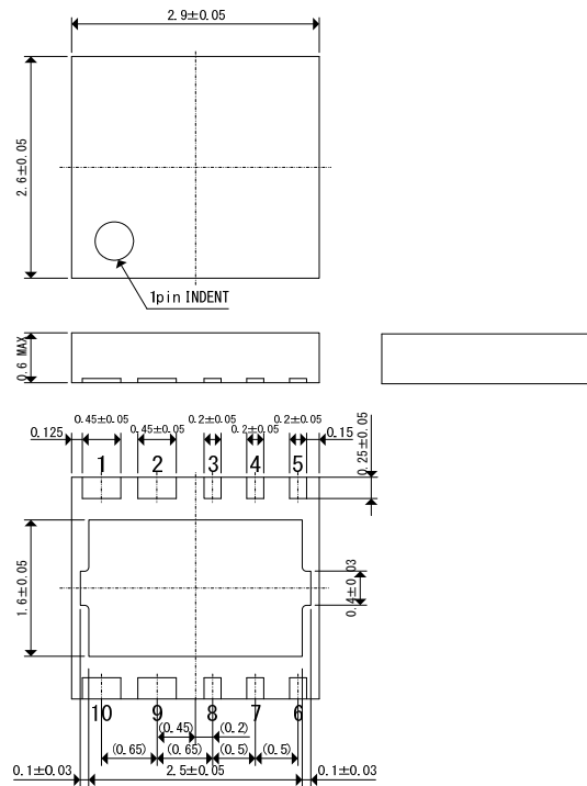
●USP-10B (unit: mm)
