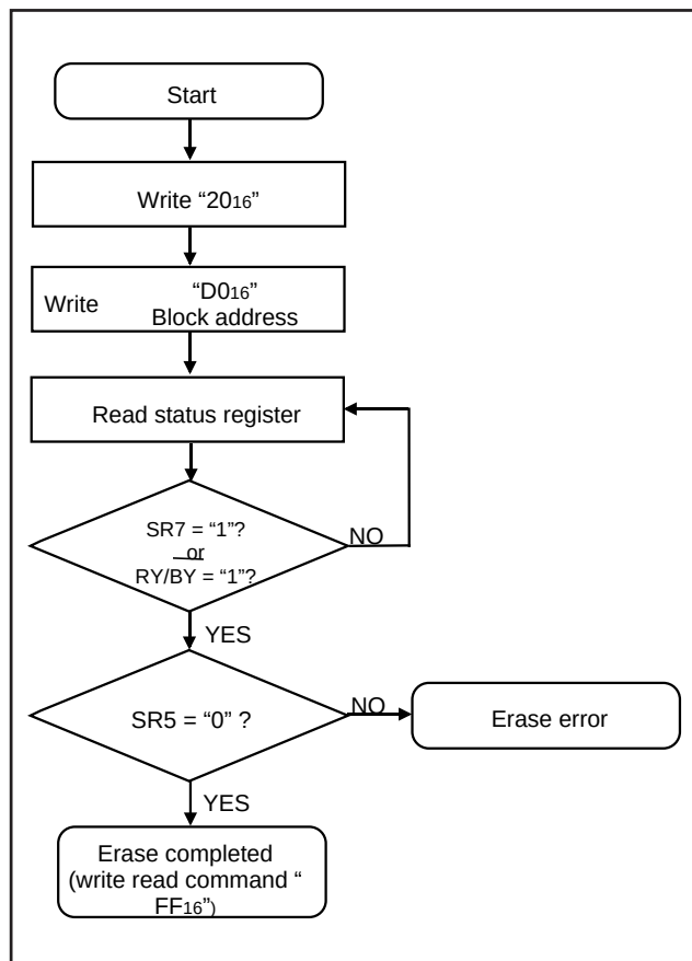
Fig. 103 Erase flowchart
