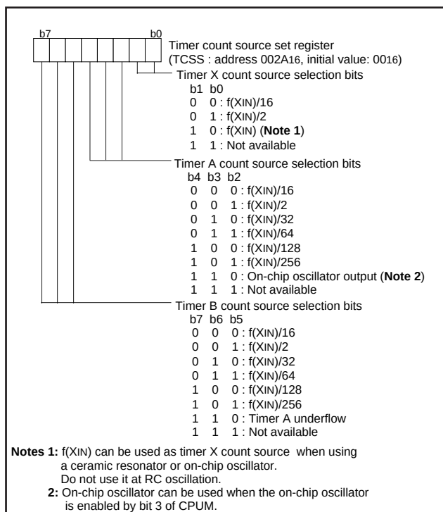
Fig. 33 Timer count source set register
