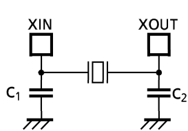
(1) High-frequency Oscillation
