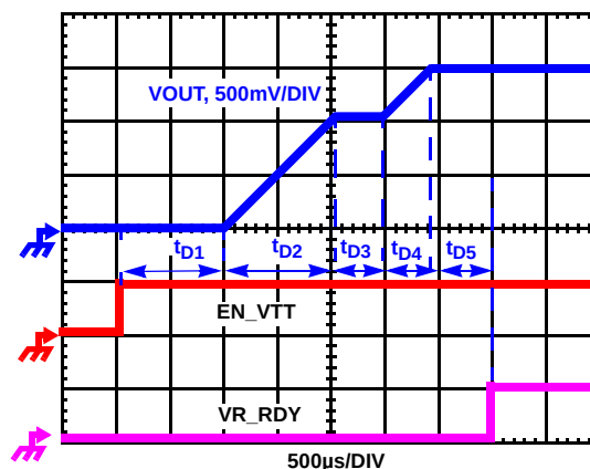
FIGURE 9. SOFT-START WAVEFORMS
