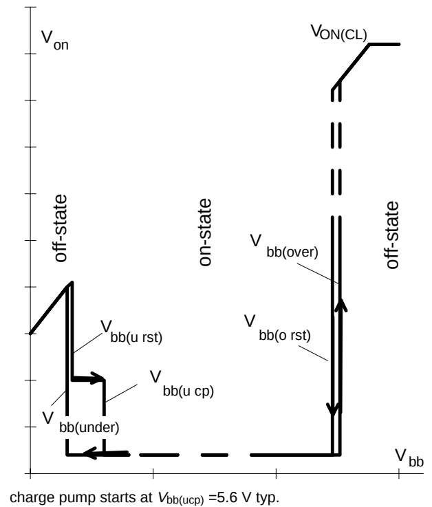
Figure 7a: Overvoltage:
