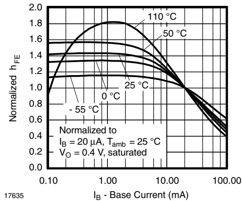
Fig. 13 - Normalized h_{FE} vs. Base Current
