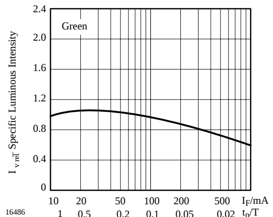
Figure 17. Specific Luminous Intensity vs. Forward Current
