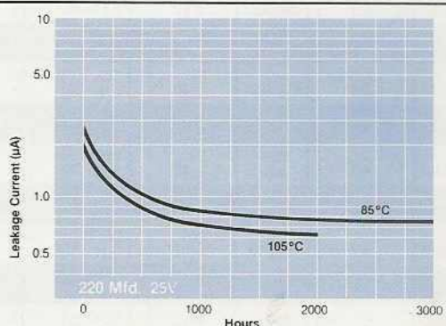
LEAKAGE CURRENT vs. TIME
