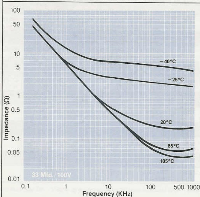
IMPEDANCE vs. FREQUENCY
