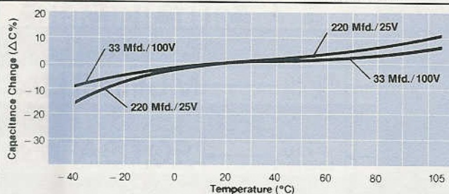
DISSIPATION FACTOR ( \tan \delta ) vs. TEMPERATURE
