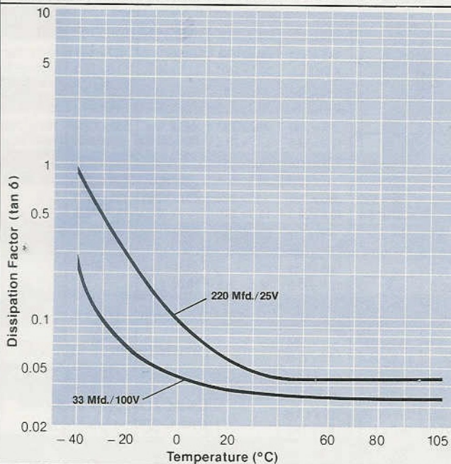
LEAKAGE CURRENT vs. TEMPERATURE
