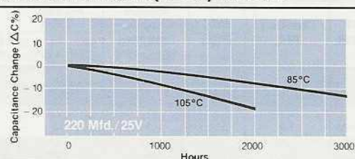
CAPACITANCE CHANGE ( \Delta C\% ) vs. TIME
