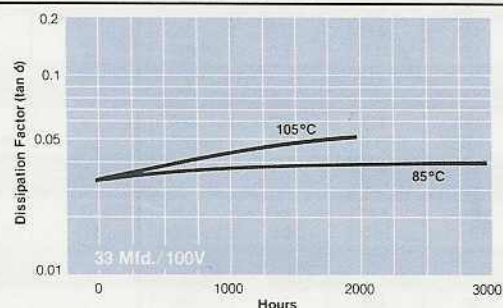
DISSIPATION FACTOR ( \tan \delta ) vs. TIME
