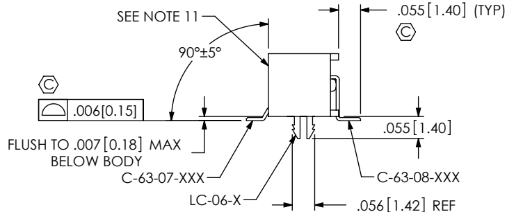
FIG 2 MMS-140-02-XXX-SH-LC SHOWN
