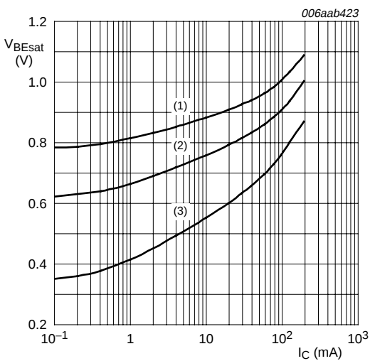
I_C/I_B = 20 (1) T_{amb} = -55\text{ }^{\circ}\text{C} (2) T_{amb} = 25\text{ }^{\circ}\text{C} (3) T_{amb} = 150\text{ }^{\circ}\text{C}
