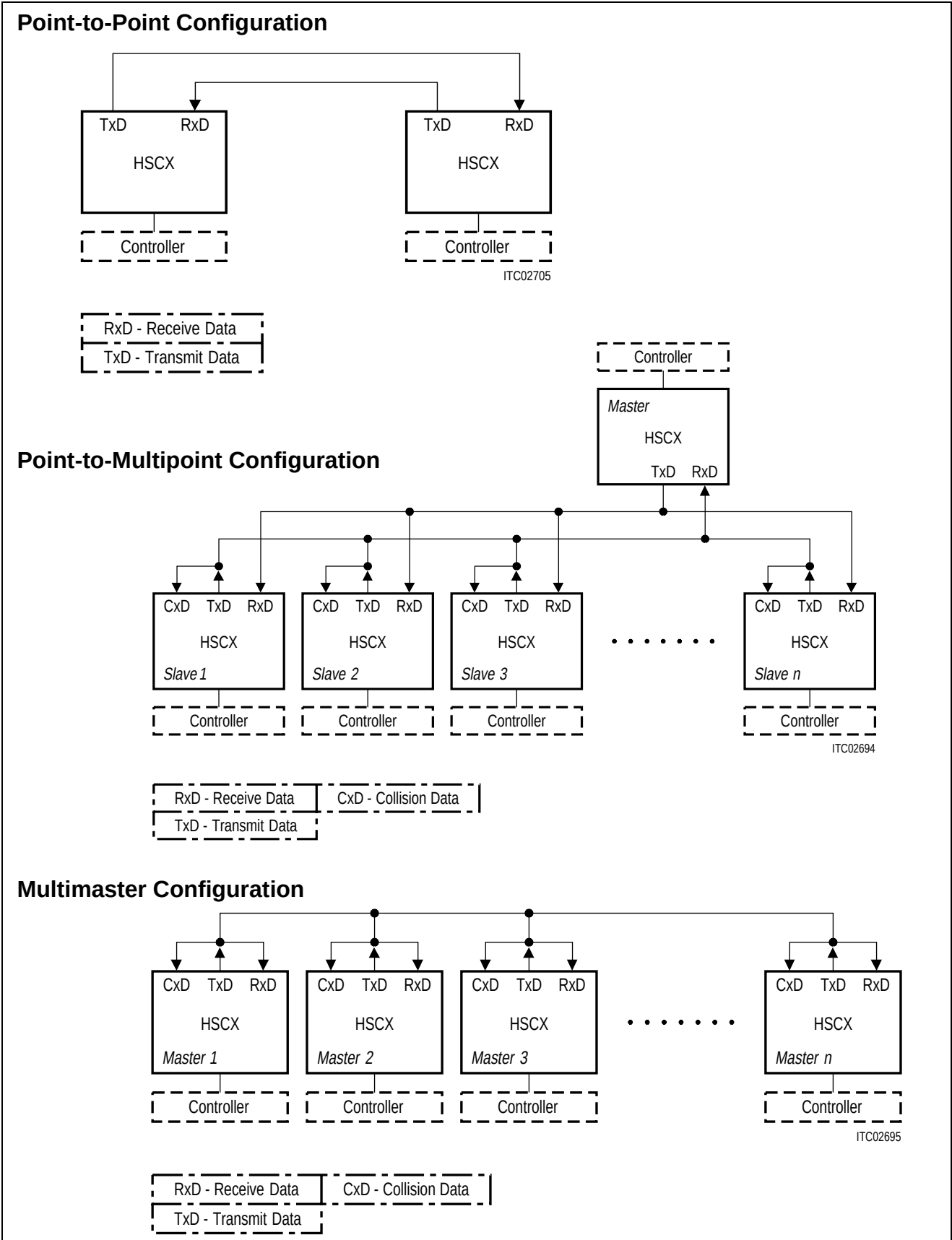
Figure 6 Link Configuration
