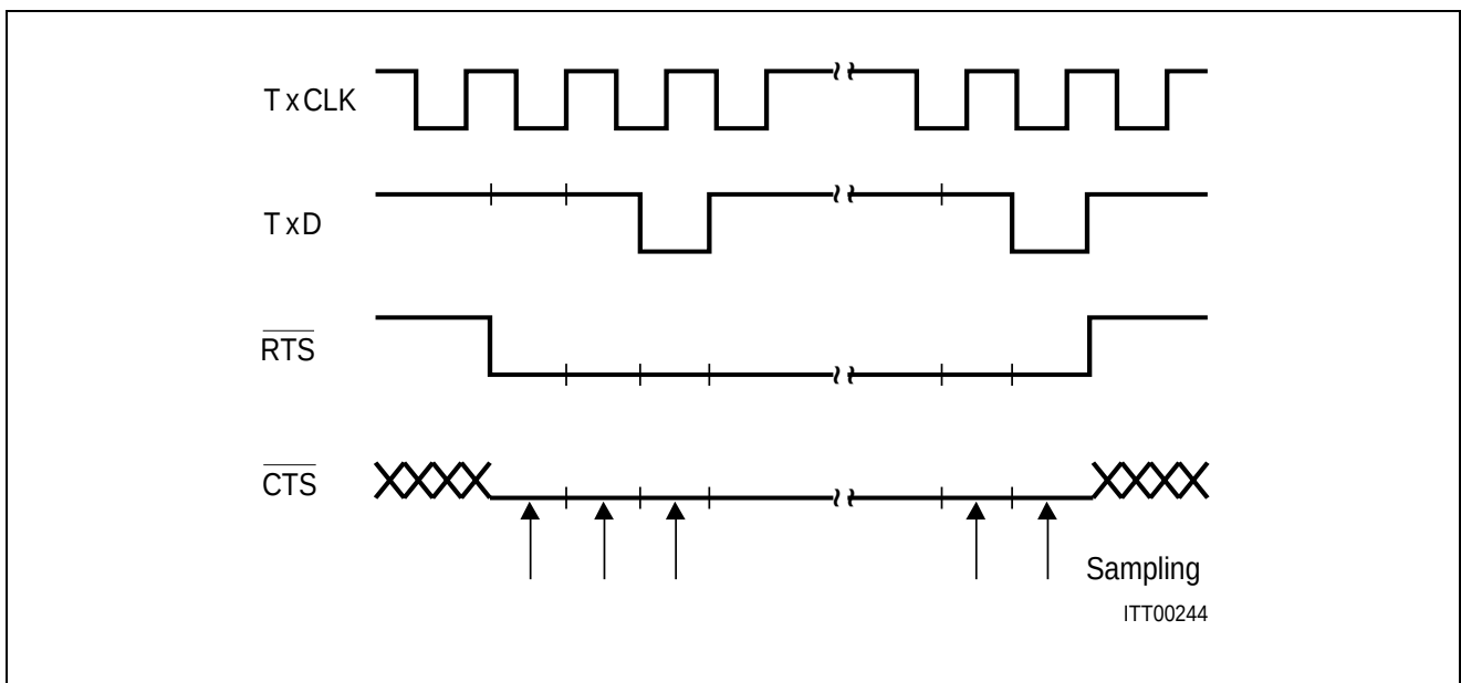
Figure 31 RTS-CTS Handshaking
