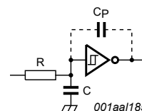
Fig. 10. Schmitt trigger driven via a high-impedance input
