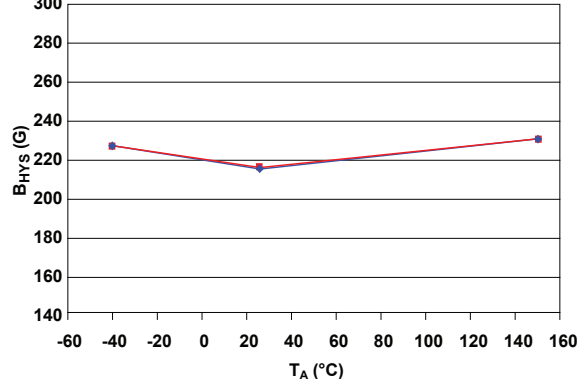
Switchpoint Hysteresis versus Temperature
