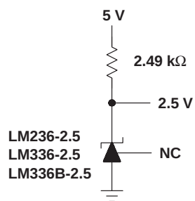
Figure 4. 2.5-V Reference
