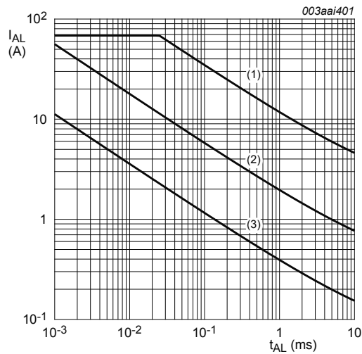
Fig. 3. Avalanche rating; avalanche current as a function of avalanche time (1) T_{j\ (init)} = 25^{\circ}C ; (2) T_{j\ (init)} = 150^{\circ}C ; (3) Repetitive Avalanche
