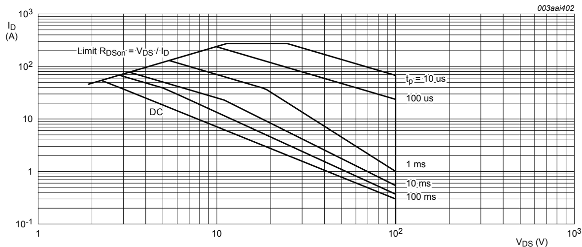
Fig. 4. Safe operating area; continuous and peak drain currents as a function of drain-source voltage T_{mb} = 25^{\circ}C ; I_{DM} is a single pulse
