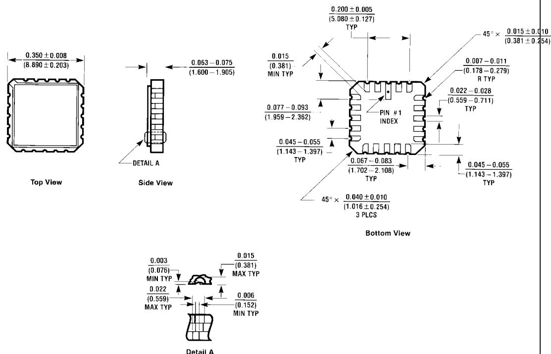
20 Lead Ceramic Leadless Chip Carrier (E) Order Number DS26LS32ME/883 NS Package Number E20A
