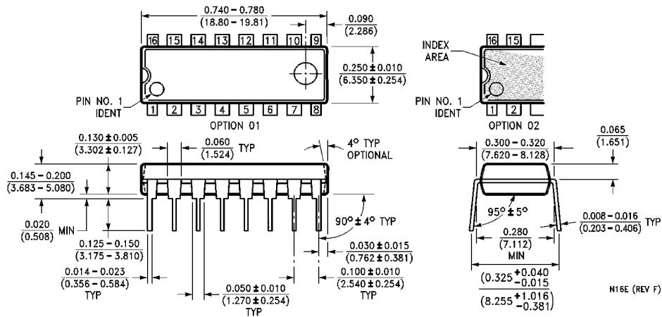
Molded Dual-In-Line Package (N) Order Number DS26LS32CN, DS26LS32ACN, or DS26LS33ACN NS Package Number N16E
