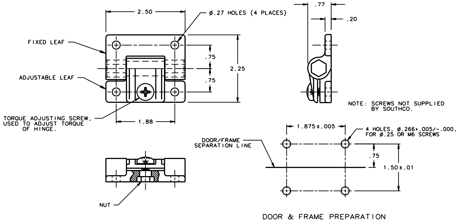
DOOR & FRAME PREPARATION
