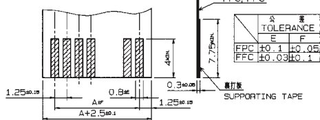
適用 FPC, FFC 寸法 RECOMMENDED APPLICABLE FPC LAYOUT
