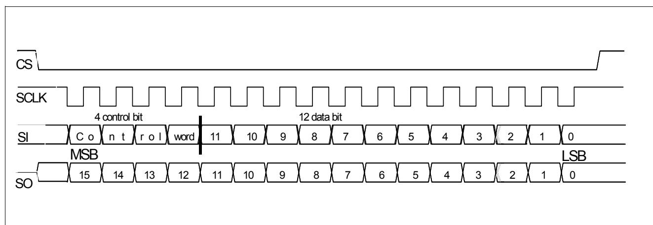
Figure 13 Serial Interface
