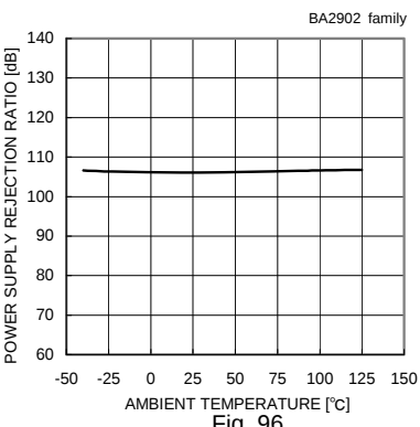
Power Supply Rejection Ratio - Ambient Temperature
