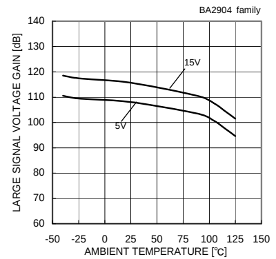
Fig. 69 Large Signal Voltage Gain - Ambient Temperature ( R_L=2[k\Omega] )
