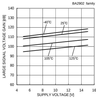
Large Signal Voltage Gain - Supply Voltage ( R_L=2[k\Omega] )
