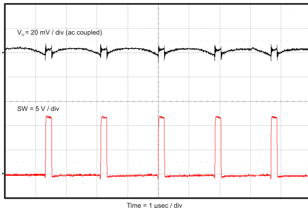
Figure 7. TPS563219EVM-663 Output Voltage Ripple, I_{OUT} = 3 A
