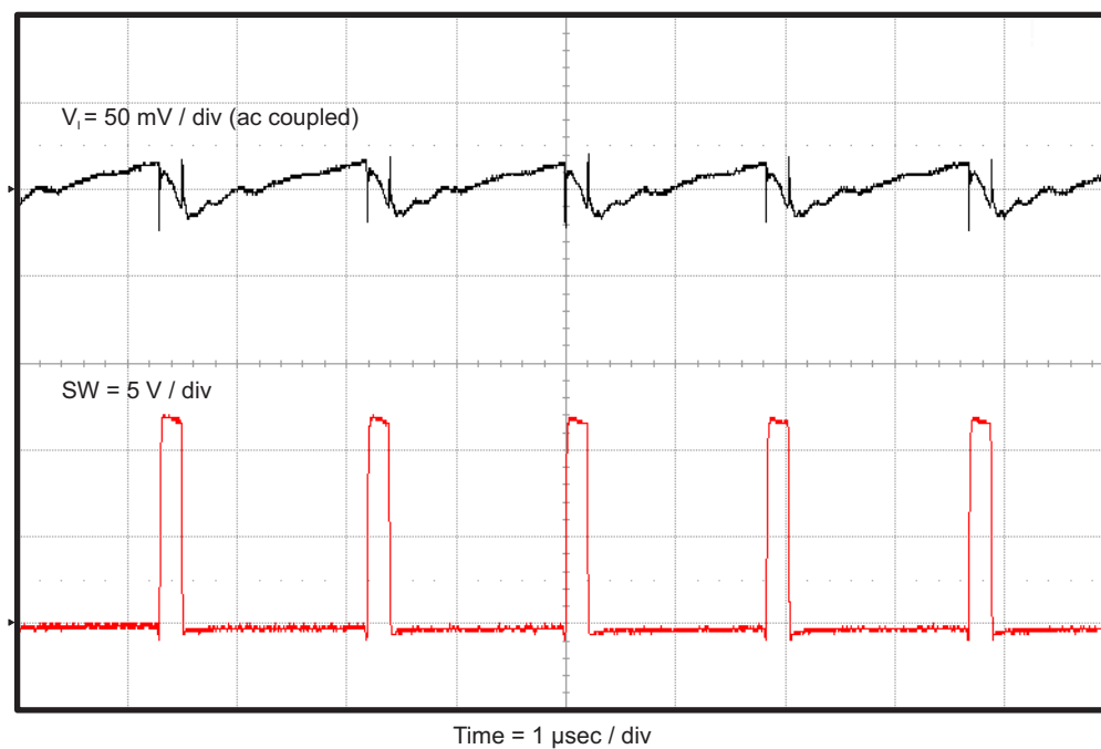
Figure 8. TPS563219EVM-663 Input Voltage Ripple, I_{OUT} = 3 A
