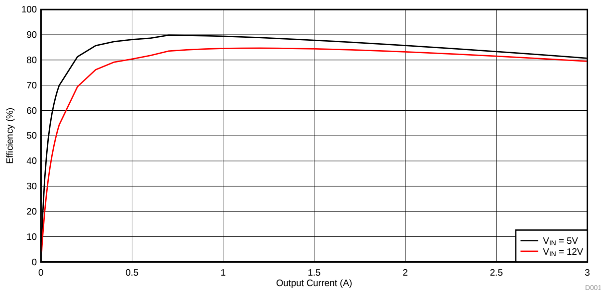
Figure 1. TPS563219EVM-663 Efficiency
